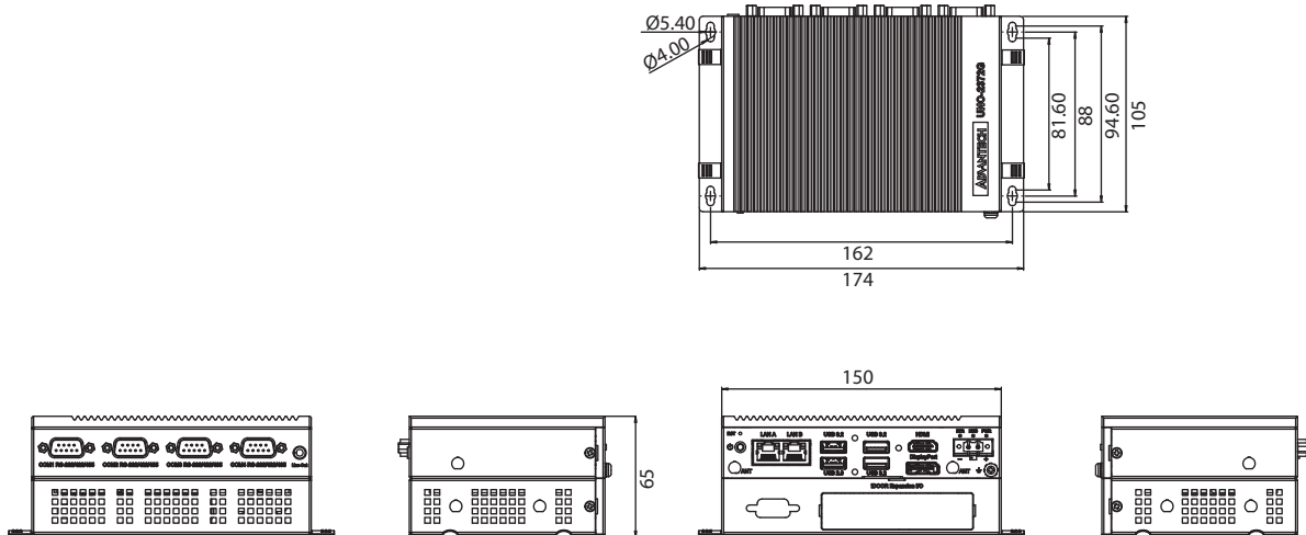
Double stack with UNO-2372G-EKCE
